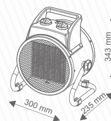
EWP 5 kW
