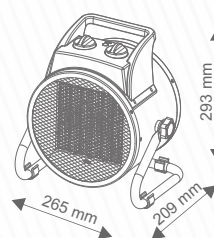
EWP 3 kW
