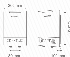
OPTISHOWER 15-21 kW
